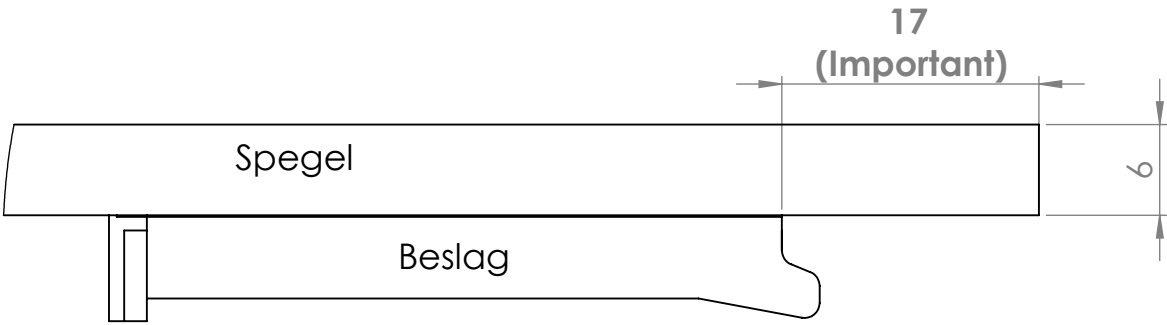
DETAIL B SCALE 2 : 1
