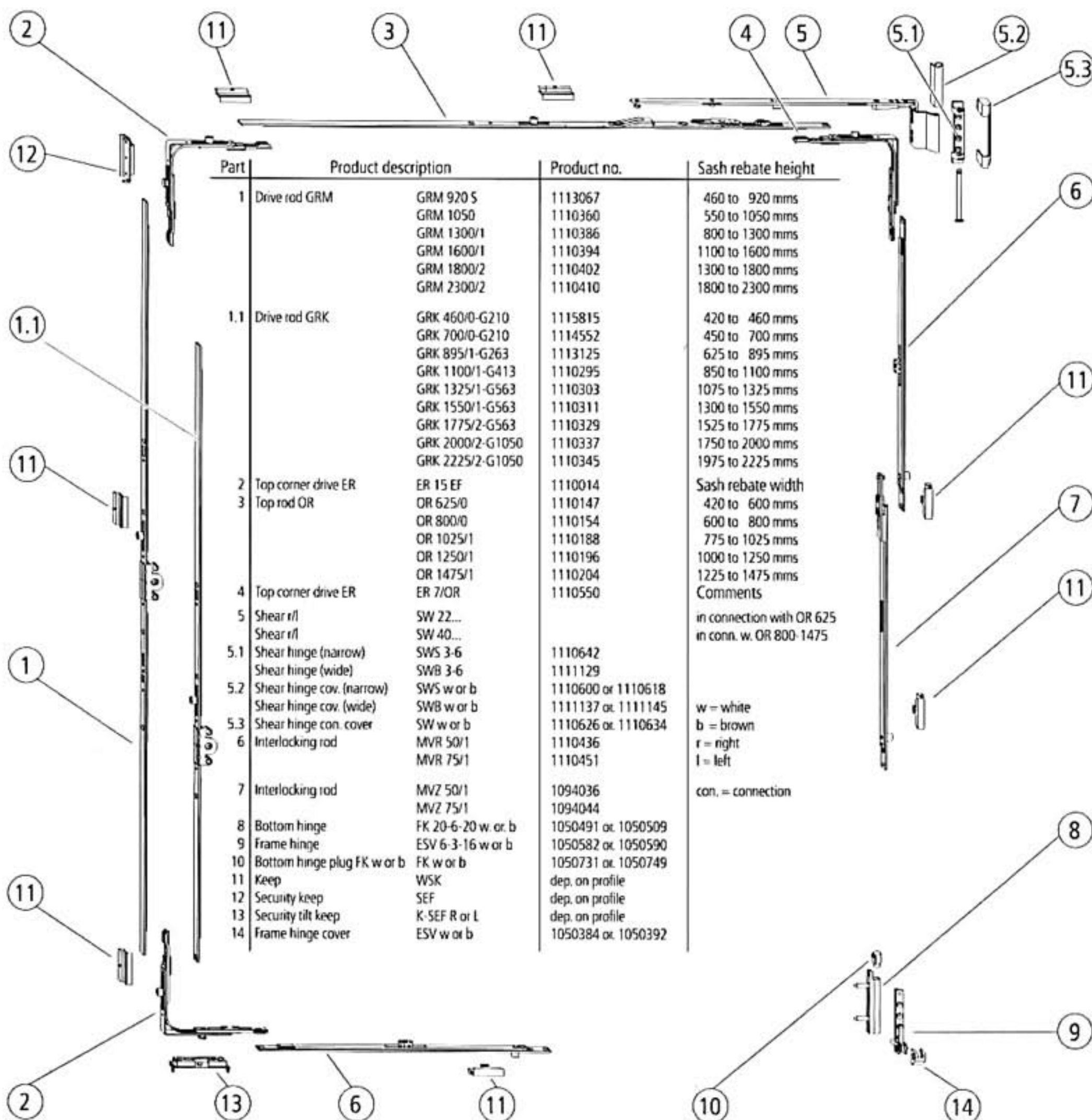
Figure 1: Overview of fittings wiht part numbers
